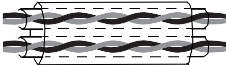
双层屏蔽 例如：JAMAK by Draka NK 电缆
